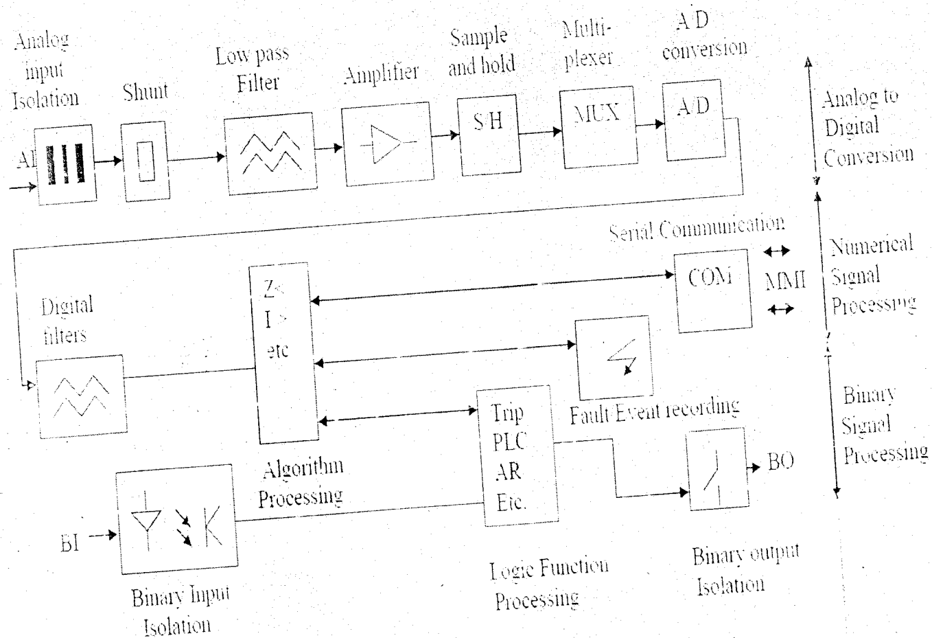
Signal flow diagram of a numerical relay
